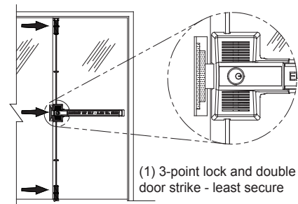
Pair of Doors - (2) 3-point locks
